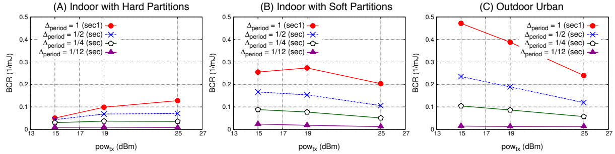
Figure 11: Impact of increasing pow_{tx} on BCR in different environments
