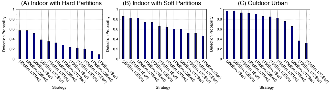
Figure 6: Strategies ranked in the descending order with respect to their corresponding detection probability in different environments
