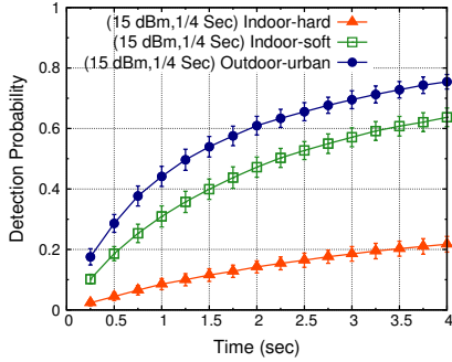
Figure 2: Same strategy in different environments. The vertical error bars present the standard deviation for the detection probability
