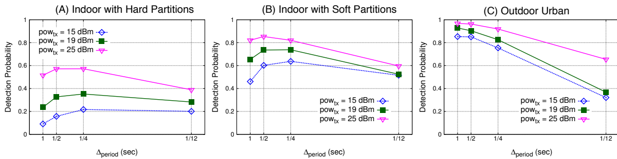
Figure 5: Impact of decreasing \Delta_{period} on the detection probability in different environments
