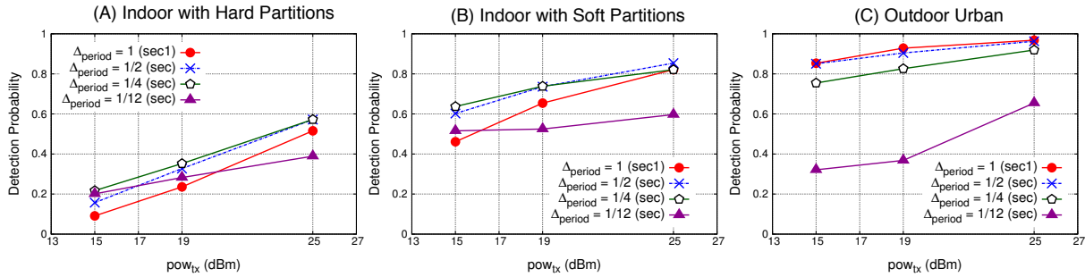
Figure 4: Impact of increasing pow_{tx} on the detection probability in different environments
