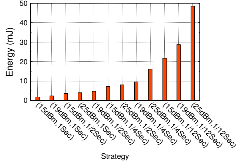
Figure 10: Strategies ranked in the ascending order with respect to their corresponding energy consumption
