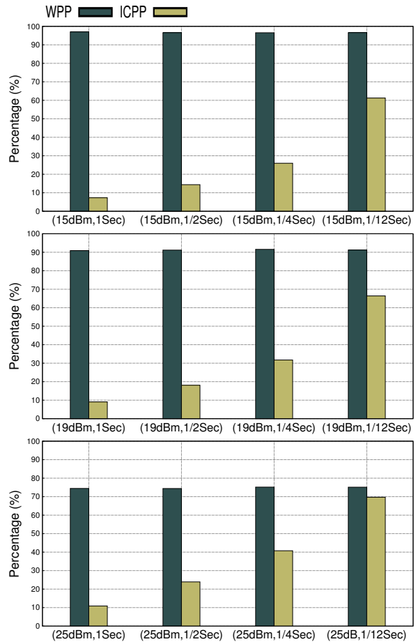
Figure 3: Values of packet dropping metrics for different strategies in the indoor with hard partitions environment
