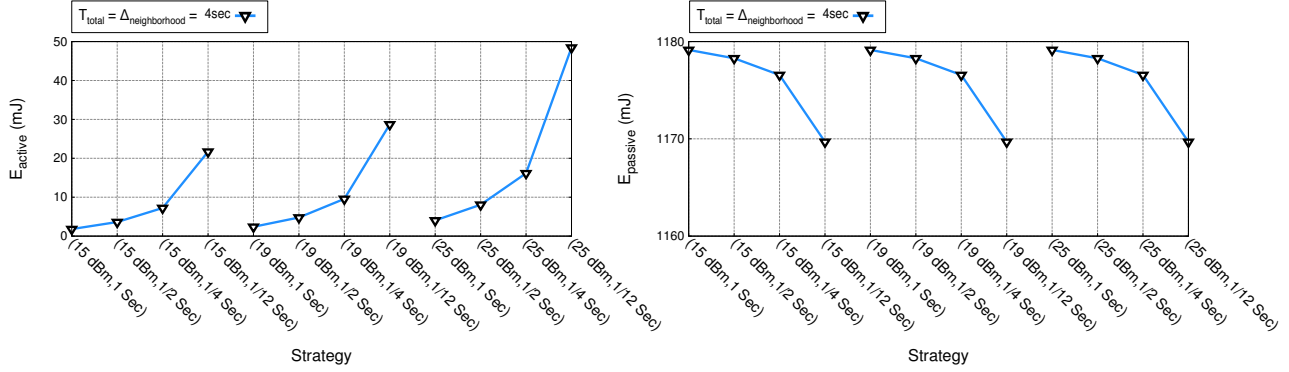
Figure 7: Variation of E_{active} and E_{passive} over different strategies when T_{total} = \Delta_{neighborhood} = 4 seconds
