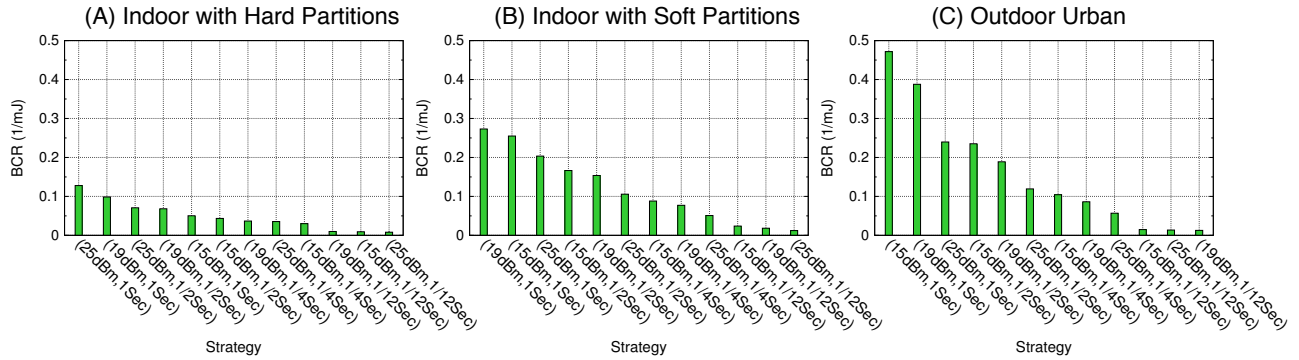
Figure 13: Strategies ranked in the descending order with respect to their corresponding BCR in different environments
