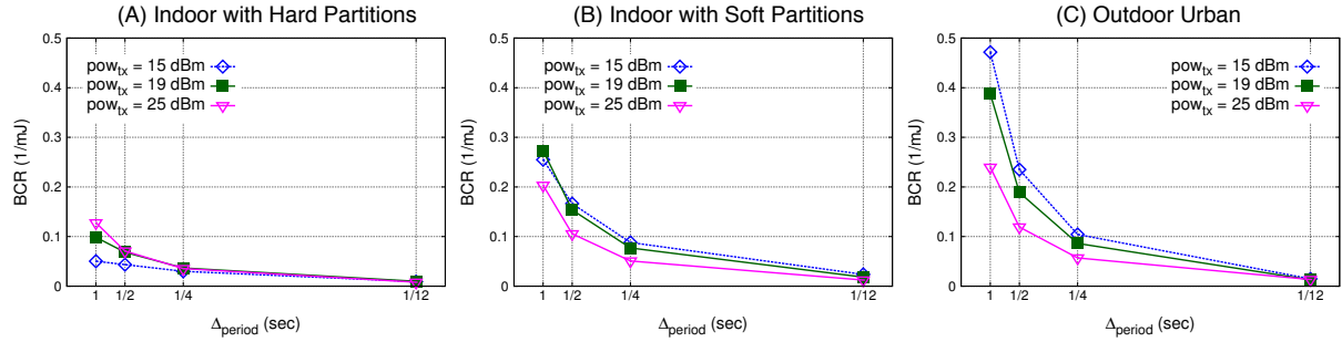
Figure 12: Impact of decreasing \Delta_{period} on BCR in different environments
