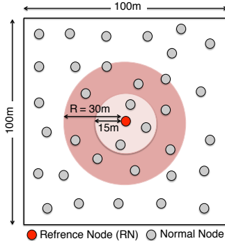
Figure 1: Simulation Map
