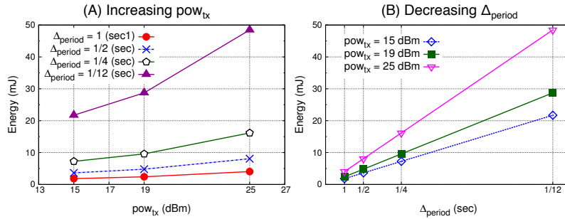
Figure 9: Impact of increasing pow_{tx} and decreasing \Delta_{period} on the energy consumption
